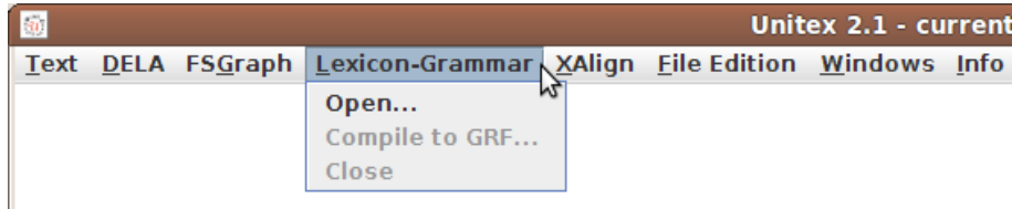
FIGURE 9.5 – Menu "Lexicon-Grammar"
