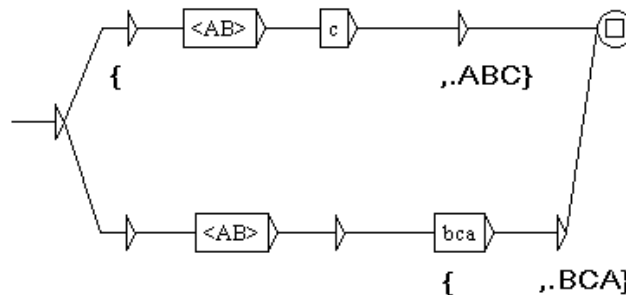
Figure 12.8: The graph tagAB
