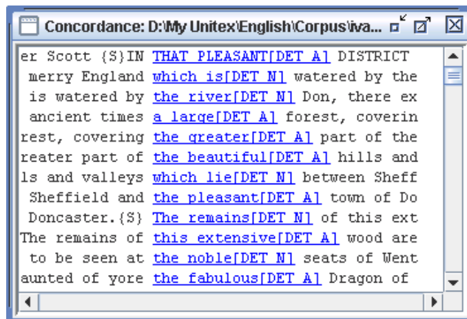
Figure 6.57: Single output for the noble
