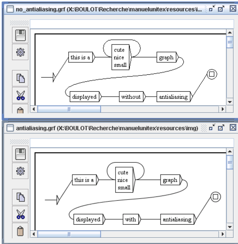
Figure 5.29: Antialiasing example
