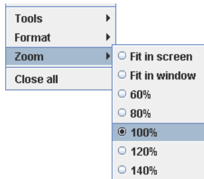
Figure 5.28: Zoom sub-menu
