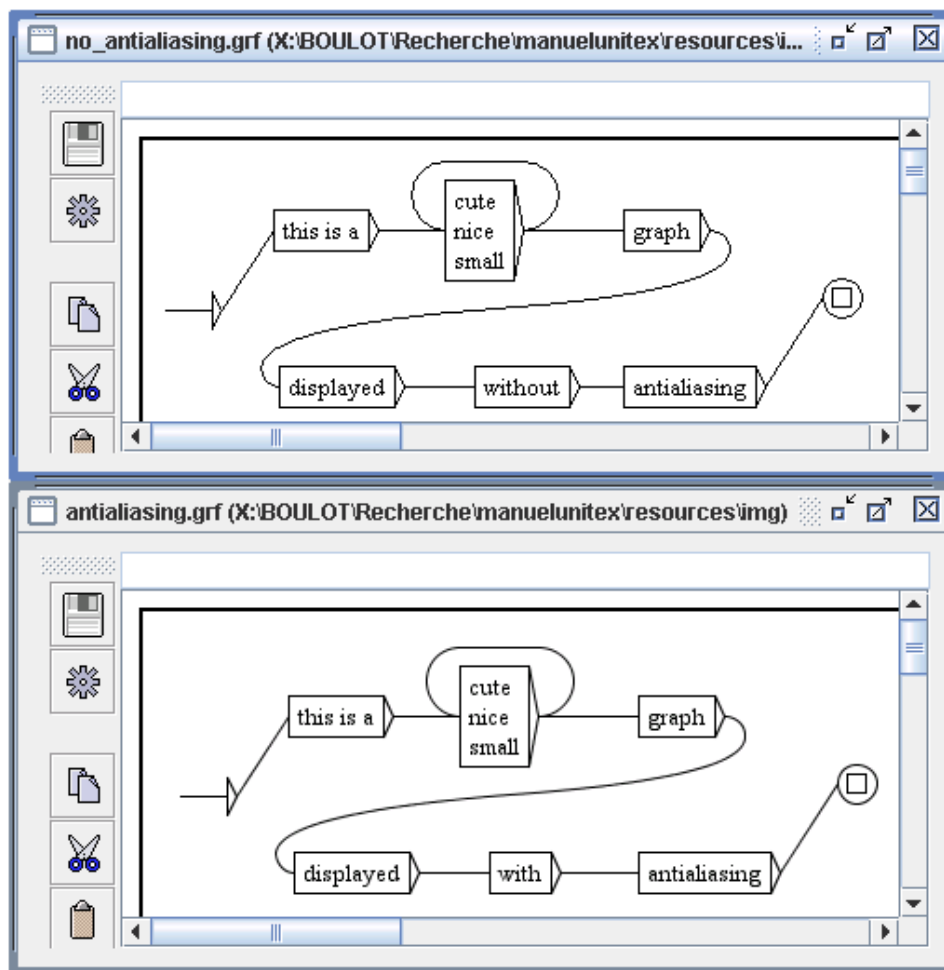
FIGURE 5.29 – Exemple d'antialiasing
