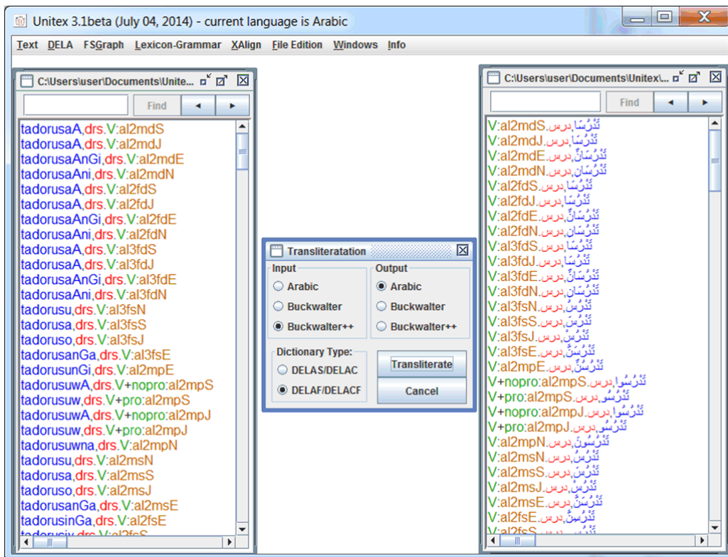
Figure 3.21: Transliteratation of a DELAF dictionary from Buckwalter++ (left) to the Arabic script (right)
