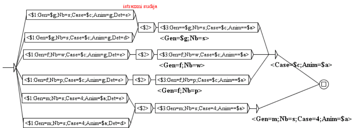
Figure 11.33: Inflection graph NC_AXNF for Serbian MWUs
