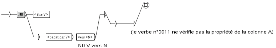
Figure 9.9: Graph generated for the verb badauder
