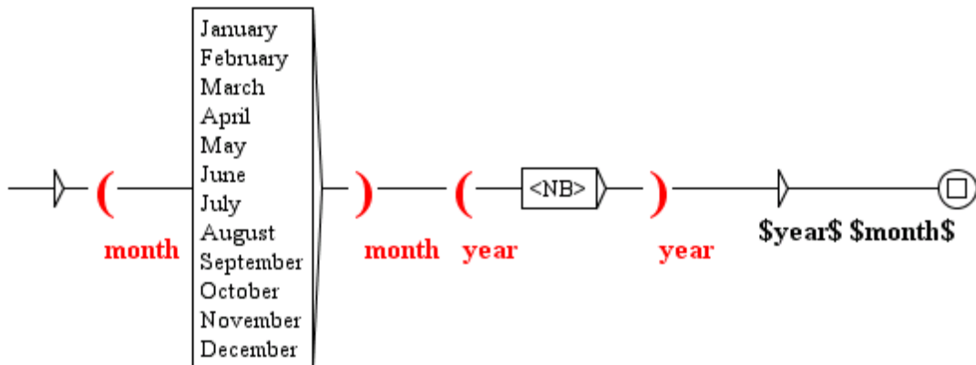
Figure 5.22: Inverting month and year in a date
