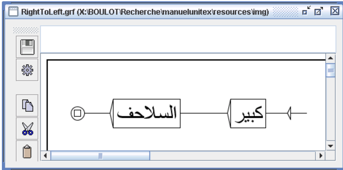
Figure 5.33: Graph with reading direction set to right to left
