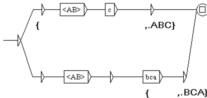
Figure 12.9: The graph tagAB
