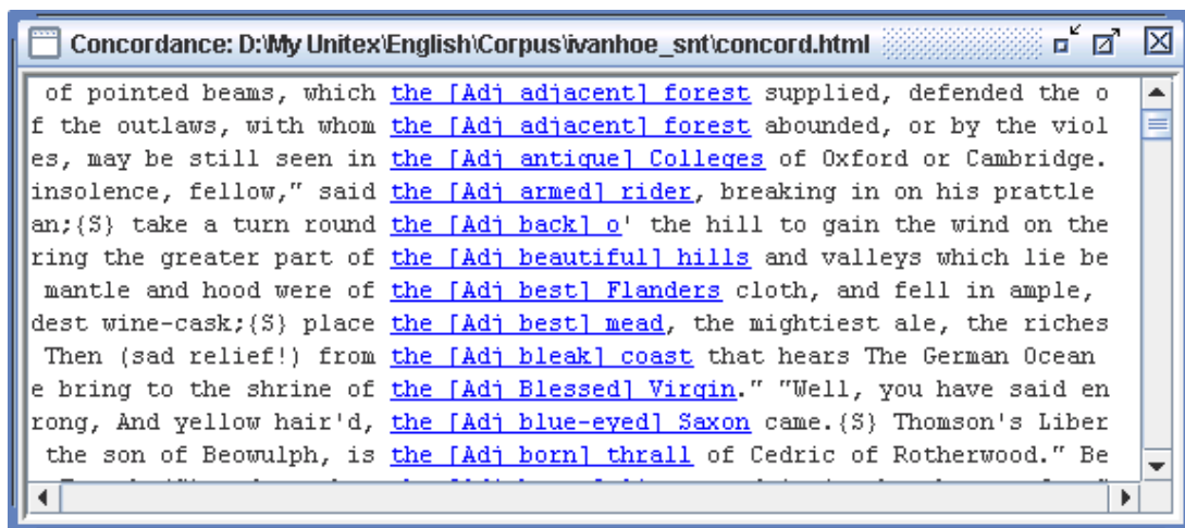
Figure 6.41: Concordance obtained in MERGE mode with the transducer of figure 6.40
