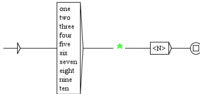
Figure 6.21: Matching a noun after a left context
