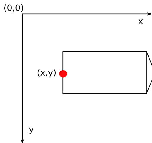
Figure 14.1: Interpretation of the coordinates of boxes
