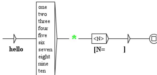
Figure 6.23: Ignored output in a left context
