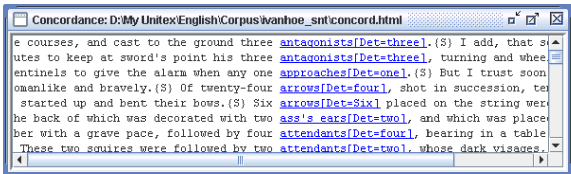
Figure 6.26: Results of the application of the grammar shown on Figure 6.25
