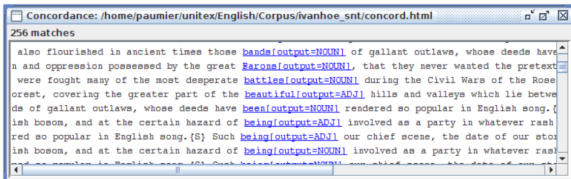
Figure 6.49: Concordance obtained with grammar of Figure 6.48
