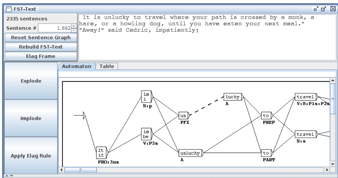
Figure 3.18: Path added by a morphological dictionary graph
