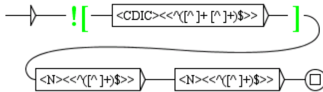
Figure 6.16: Advanced use of right contexts
