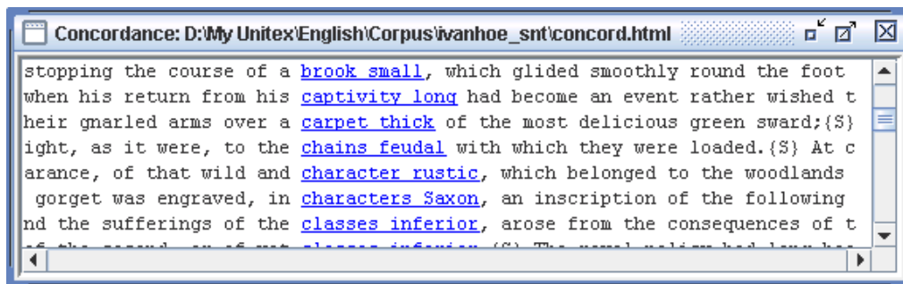
Figure 6.46: Result of the application of the transducer in figure 6.45
