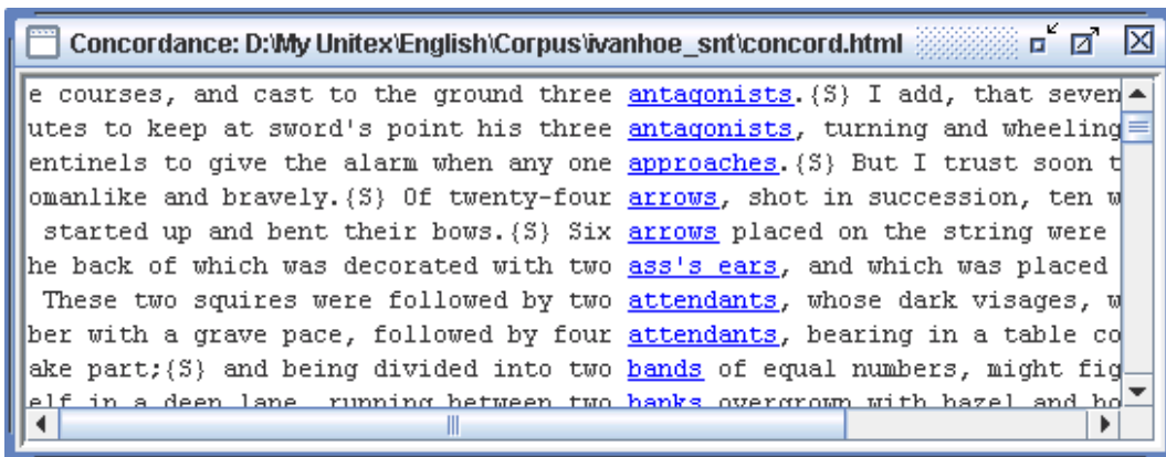
Figure 6.22: Results of the application of the grammar shown on Figure 6.21
