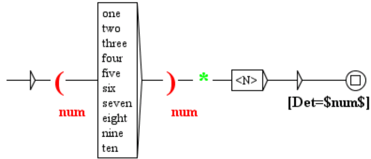
Figure 6.25: Using a variable in a left context
