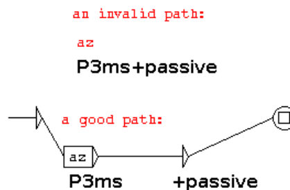
Figure 3.10: An inflection grammar with a semantic code
