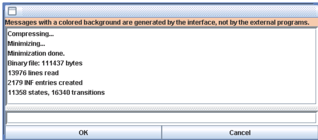
Figure 3.13: Results of a compression
