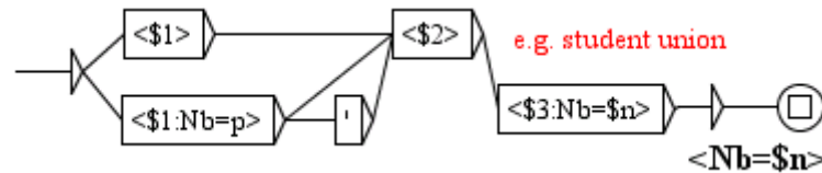
Figure 11.8: Inflection graph for student union
