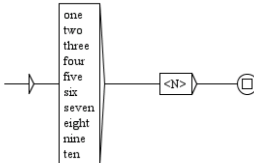
Figure 6.19: Matching a noun that occurs after a numerical determiner
