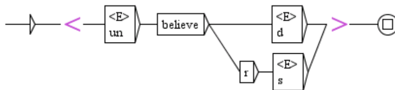
Figure 6.30: Example of morphological zone in a grammar
