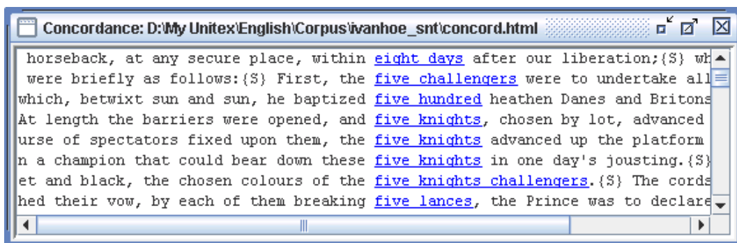
Figure 6.20: Results of the application of the grammar shown on Figure 6.19
