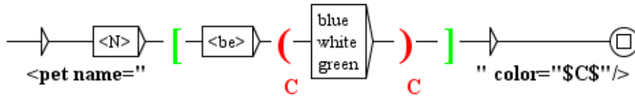
Figure 6.18: Variable defined inside a right context
