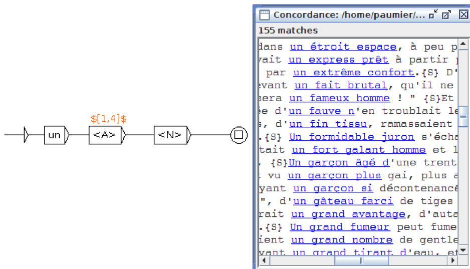
Figure 6.11: use of interval to match several consecutive tokens
