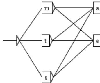
Figure 3.12: Representation of a minimal automaton
