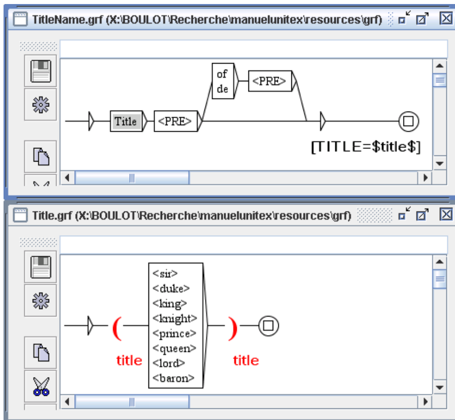
Figure 6.43: Definition of a variable in a subgraph
