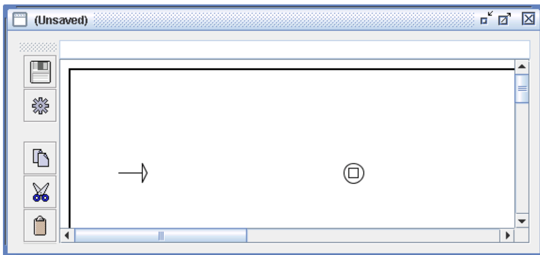
Figure 5.2: Empty graph
