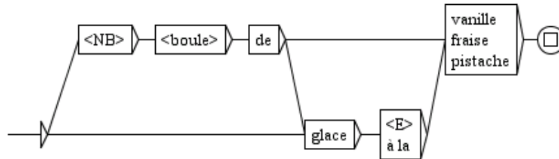
Figure 6.37: Sample graph
