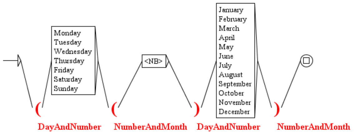
Figure 6.47: Overlapping variables
