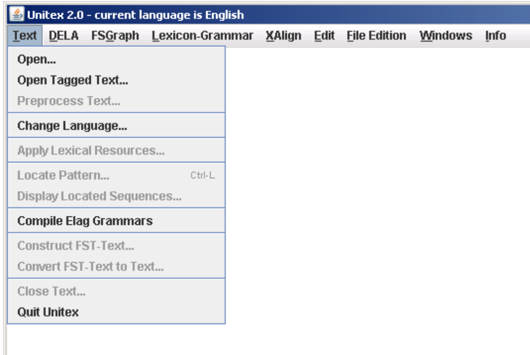
Figure 2.6: Text Menu
