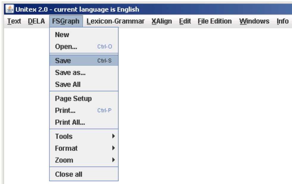
Figure 5.1: FSGraph menu
