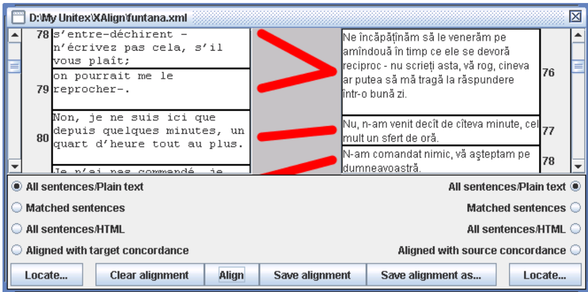
Figure 9.4: Aligned sentences
