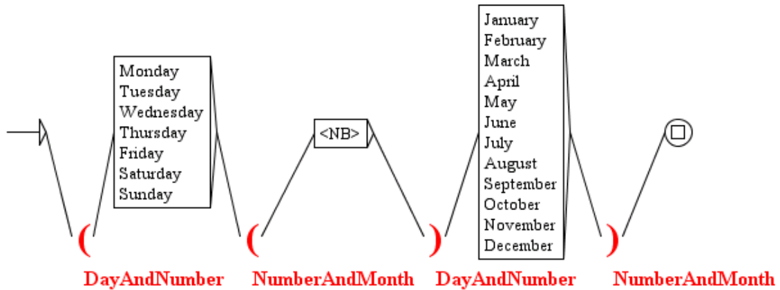
Figure 6.46: Overlapping variables
